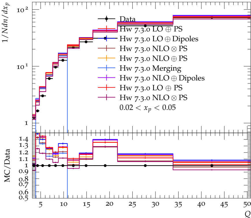
Current hemisphere fragmentation as a function of Q
