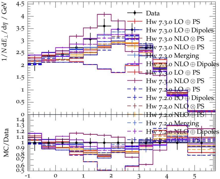
Transverse energy flow for \langle x \rangle = 0.0043 , \langle Q^2 \rangle = 175 \text{ GeV}^2
