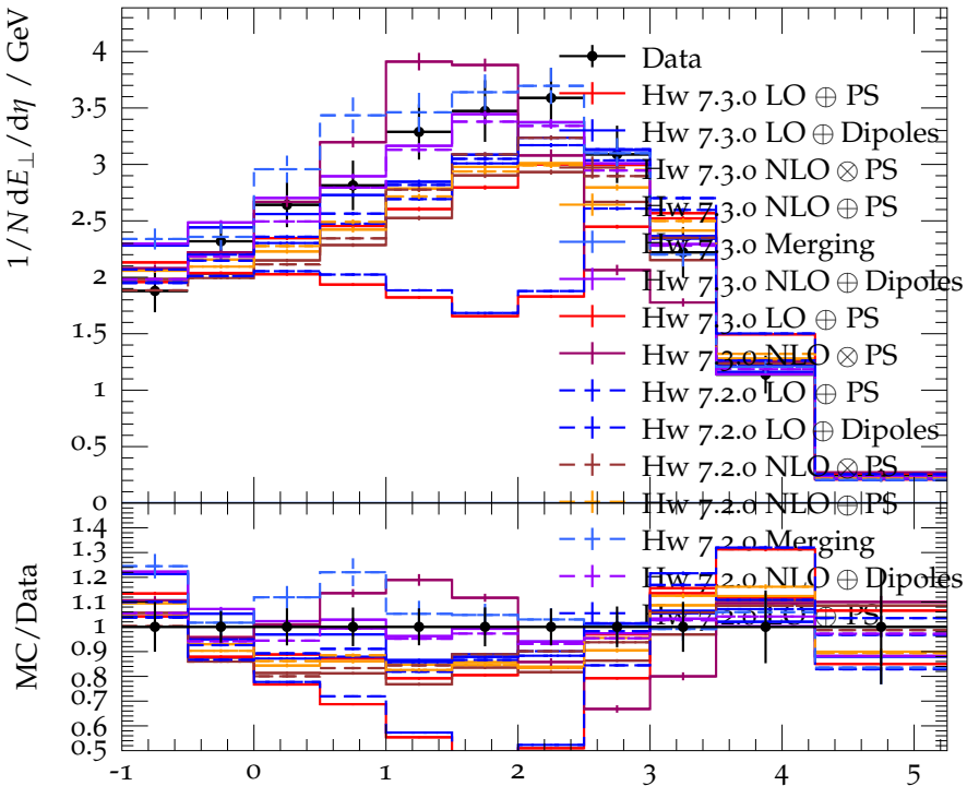
Transverse energy flow for \langle x \rangle = 0.01, \langle Q^2 \rangle = 253 \text{ GeV}^2
