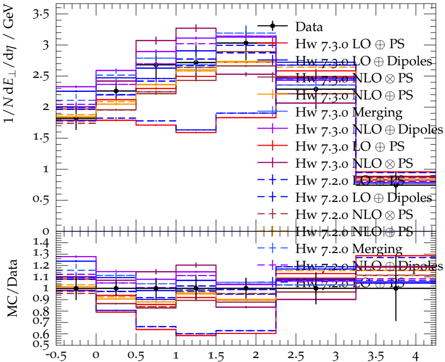
Transverse energy flow for \langle x \rangle = 0.026 , \langle Q^2 \rangle = 283 \text{ GeV}^2
