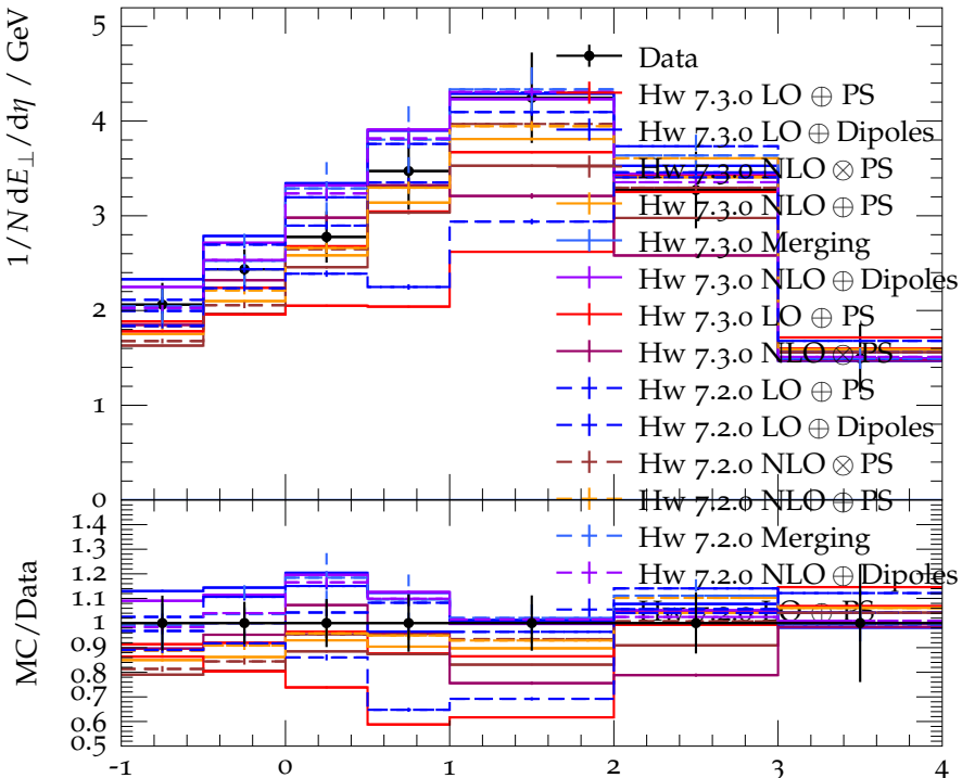
Transverse energy flow for \langle x \rangle = 0.11, \langle Q^2 \rangle = 2200 \text{ GeV}^2
