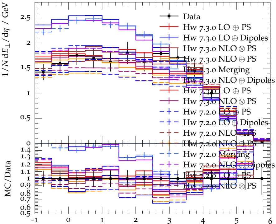
Transverse energy flow for \langle Q^2 \rangle = 2.5 - 5 \text{ GeV}^2
