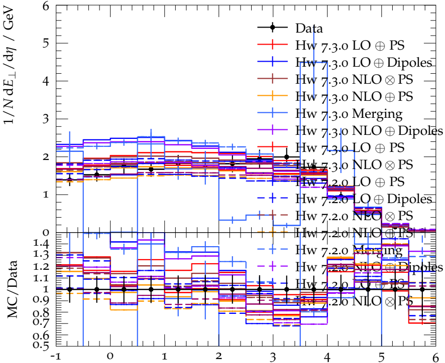
Transverse energy flow for \langle Q^2 \rangle = 5 - 10 \text{ GeV}^2
