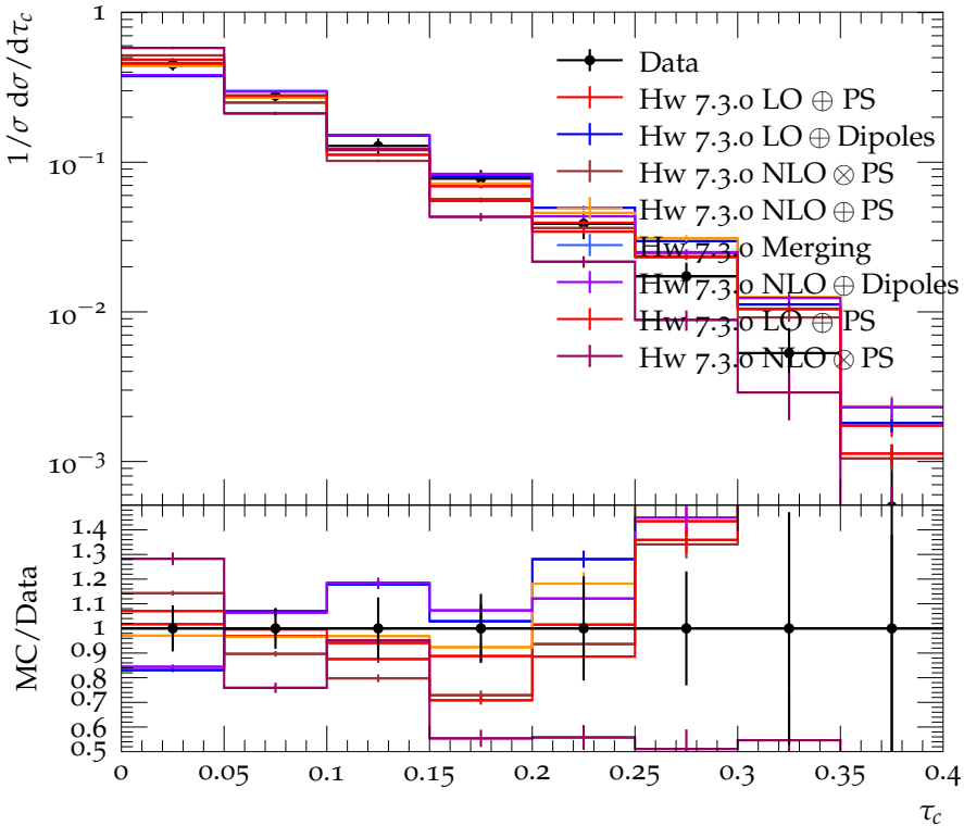
\tau_c distribution for \langle Q \rangle \geq 58\text{GeV}
