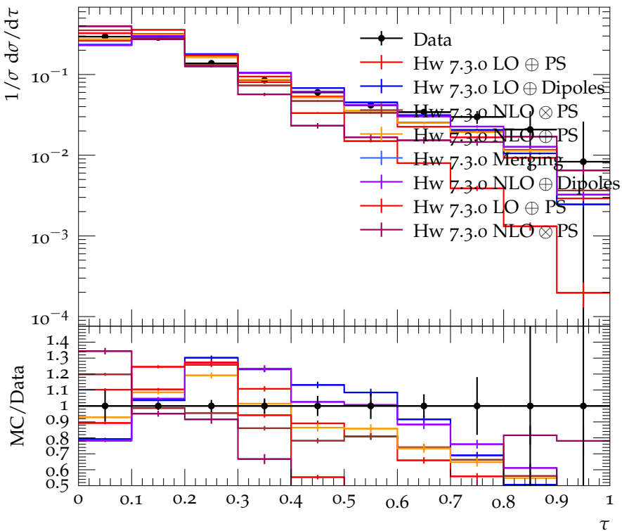
\tau distribution for \langle Q \rangle \leq 24\text{GeV}
