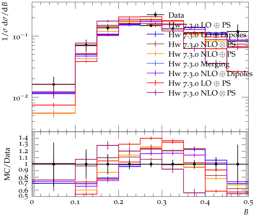
B distribution for \langle Q \rangle = 15\text{GeV}
