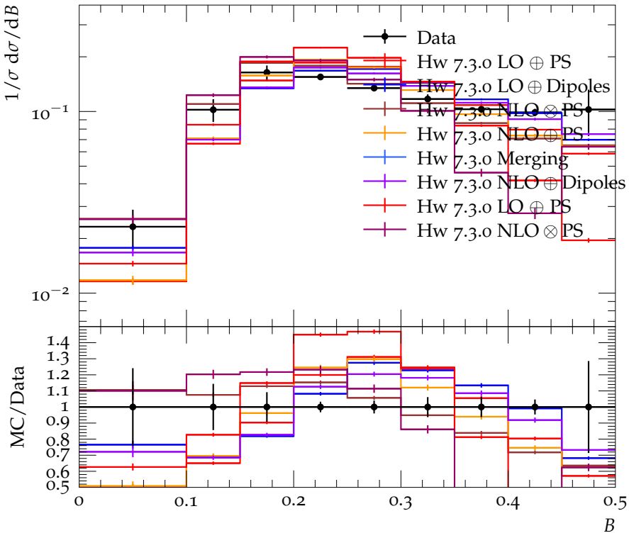
B distribution for \langle Q \rangle \leq 18\text{GeV}
