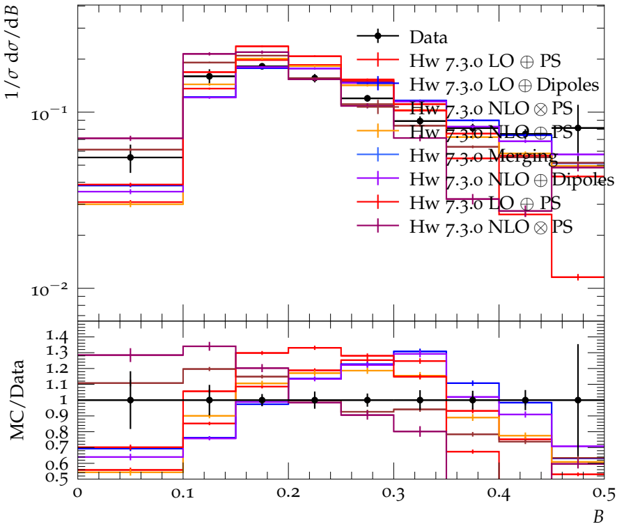
B distribution for \langle Q \rangle = 24\text{GeV}
