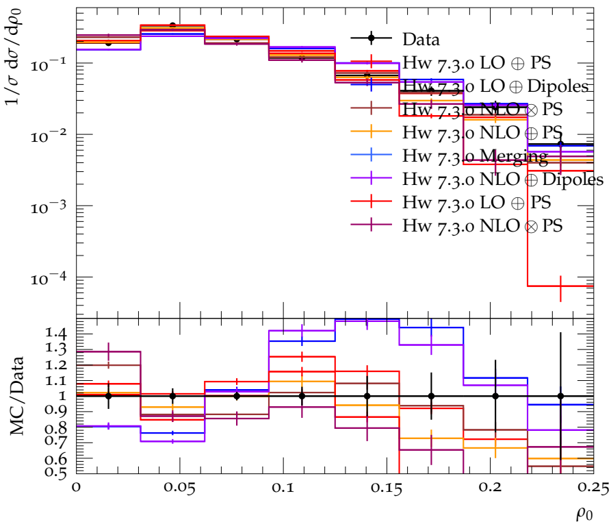
\rho_0 distribution for \langle Q \rangle = 15\text{GeV}
