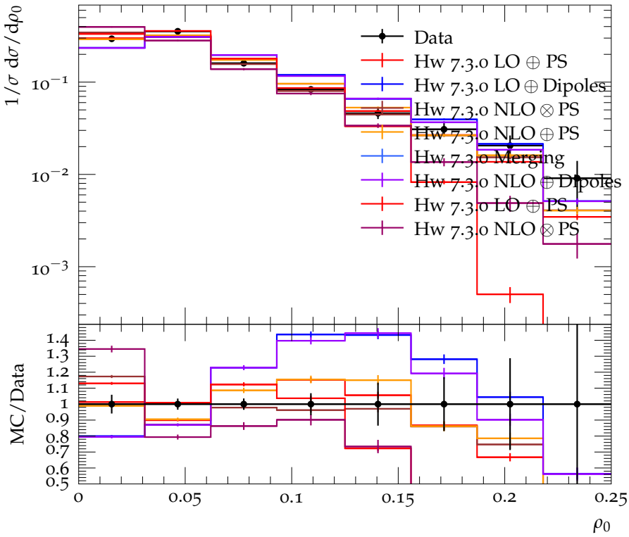
\rho_0 distribution for \langle Q \rangle \geq 24\text{GeV}
