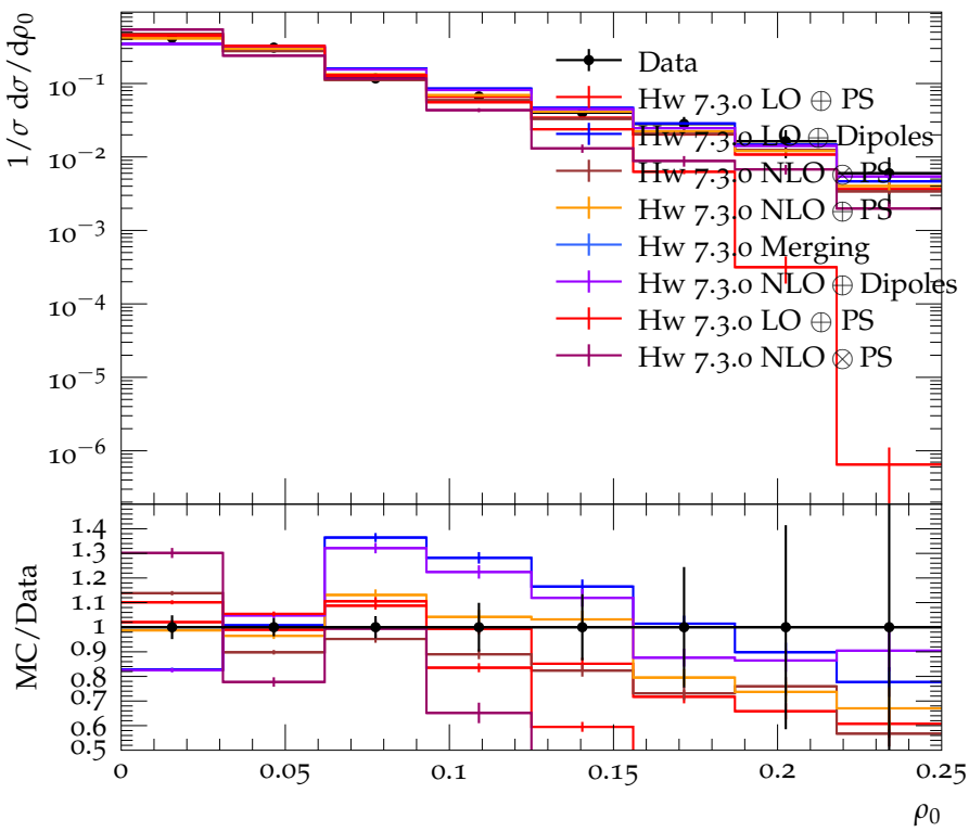
\rho_0 distribution for \langle Q \rangle = 37\text{GeV}
