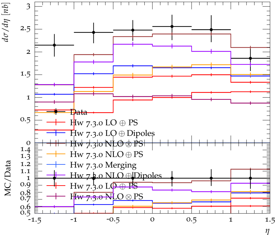
d\sigma/d\eta for inclusive D^{*\pm} production in the vis. kin. region
