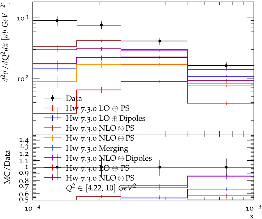
d^2\sigma/dQ^2 dx for inclusive D^{*\pm} production in bins of Q^2 and x
