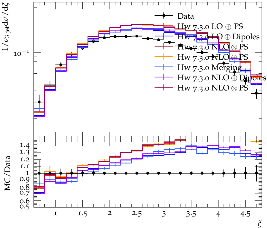
Log Scaled momentum fraction for K_{\zeta}^0 in 1st jet (3-jet events)
