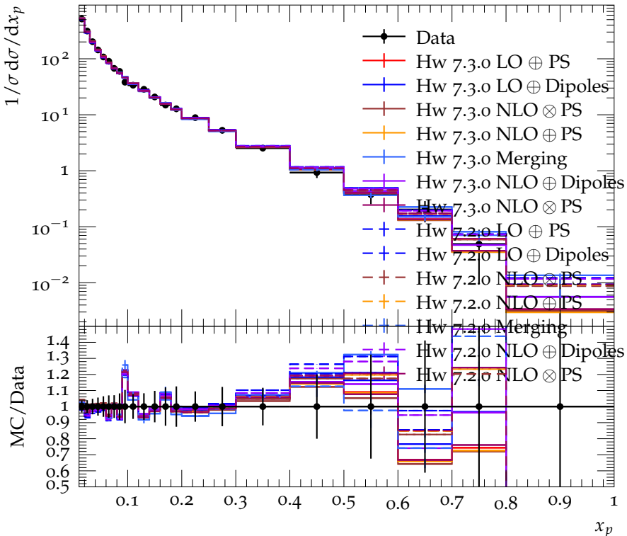
Charged particle spectrum ( E_{\text{CMS}} = 161 \text{ GeV} )
