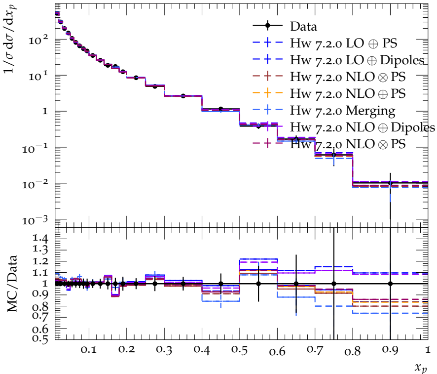
Charged particle spectrum ( E_{\text{CMS}} = 196 \text{ GeV} )
