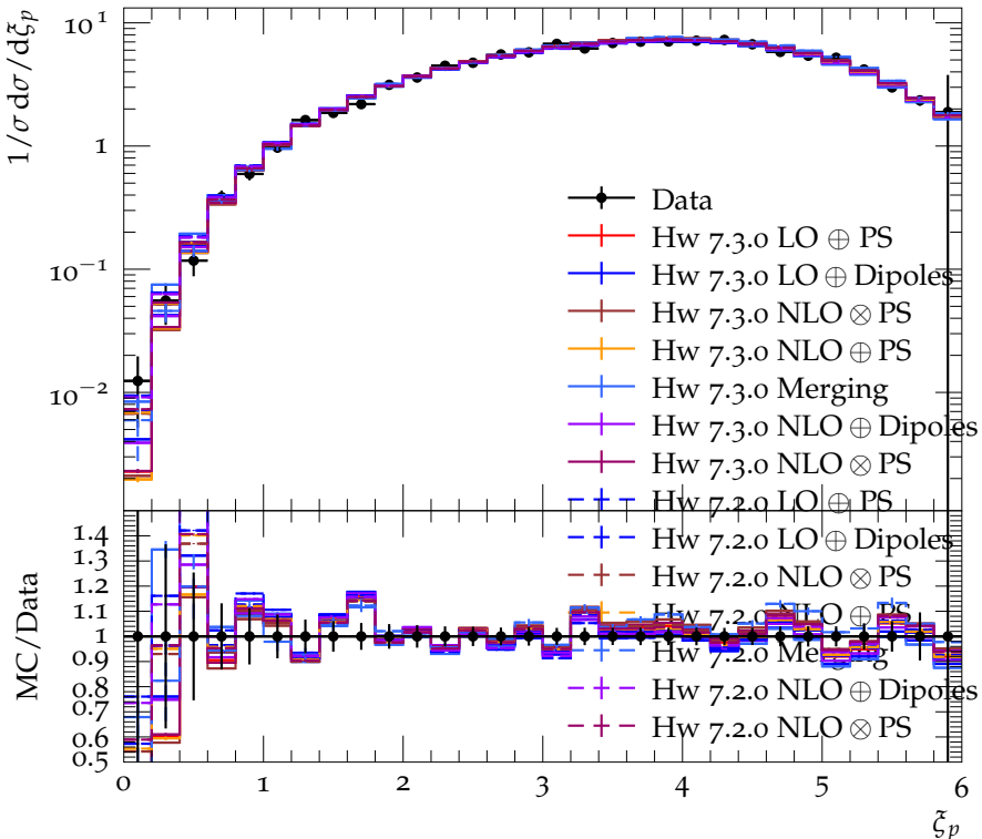
Charged particle spectrum ( E_{\text{CMS}} = 133 \text{ GeV} )
