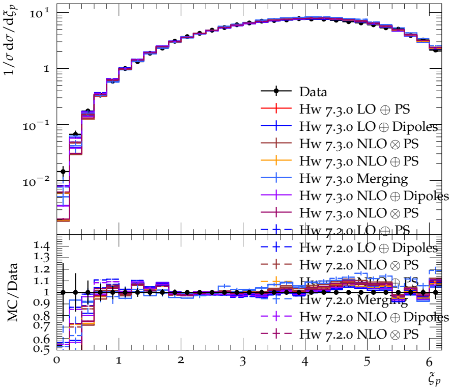
Charged particle spectrum ( E_{\text{CMS}} = 189 \text{ GeV} )
