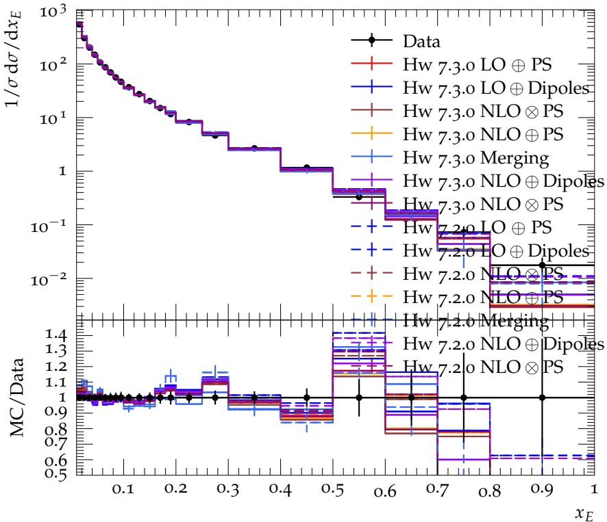
Charged particle spectrum ( E_{\text{CMS}} = 206 \text{ GeV} )
