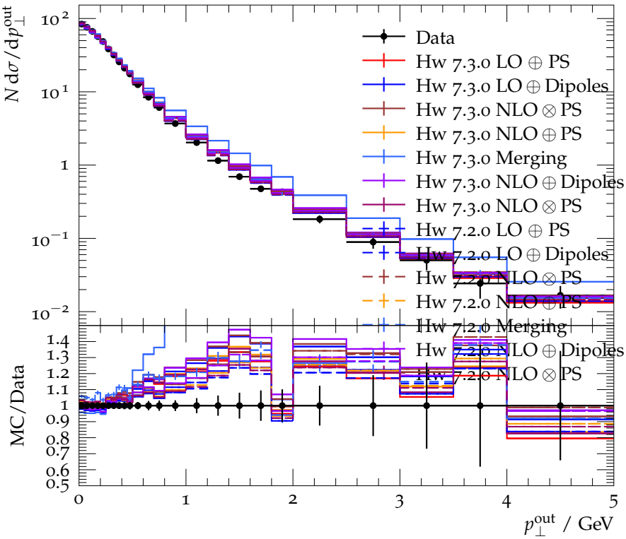
Out-of-plane p_{\perp} in GeV w.r.t. thrust axes ( E_{\text{CMS}} = 206 \text{ GeV} )
