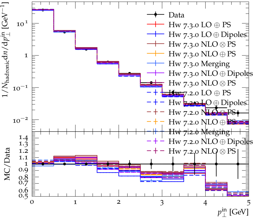
p_{\perp}^{\text{in}} for charged particles w.r.t the sphericity axis
