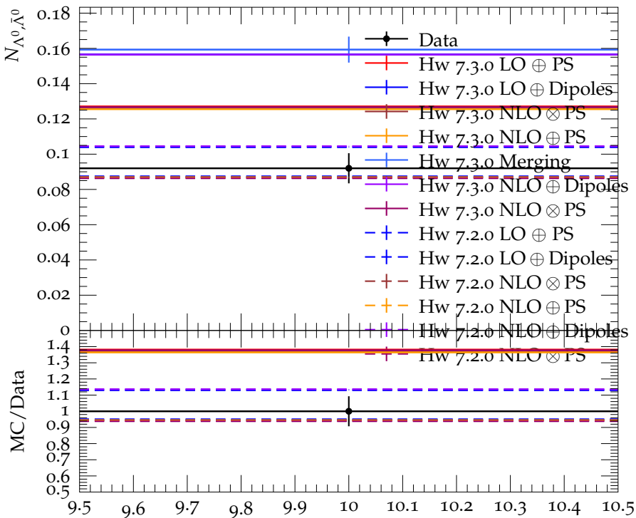
Multiplicity of \Lambda^0, \bar{\Lambda}^0 in the continuum (10 GeV)
