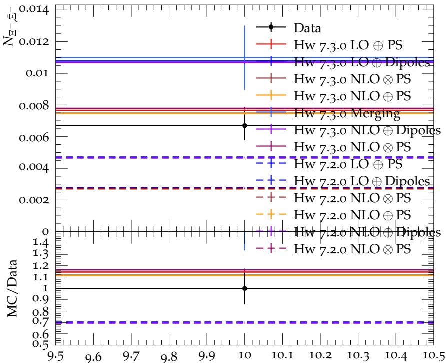
Multiplicity of \Xi^- , \bar{\Xi}^- in the continuum (10 GeV)
