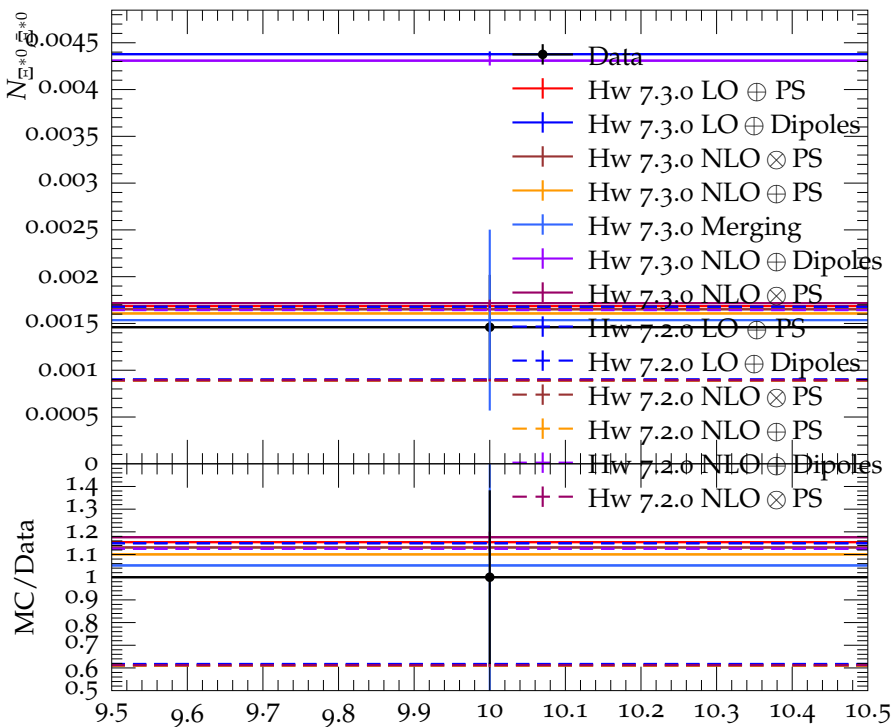
Multiplicity of \Xi^{*0}, \bar{\Xi}^{*0} in the continuum (10 GeV)
