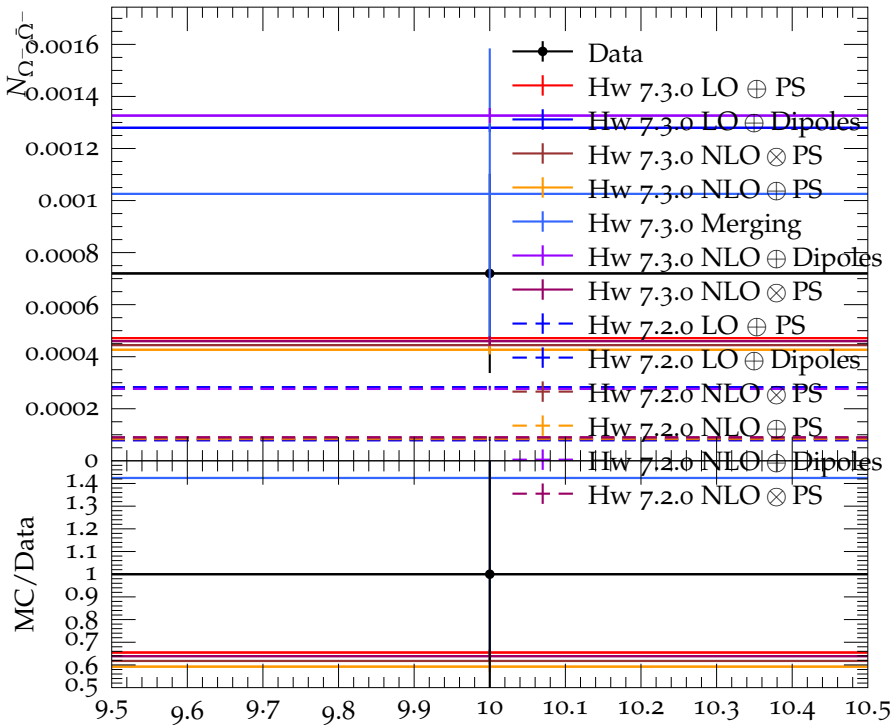
Multiplicity of \Omega^- , \bar{\Omega}^- in the continuum (10 GeV)
