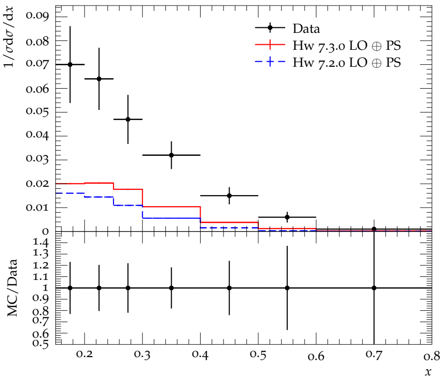
Spectrum of \Xi^- , \bar{\Xi}^- in Y(1S) decays
