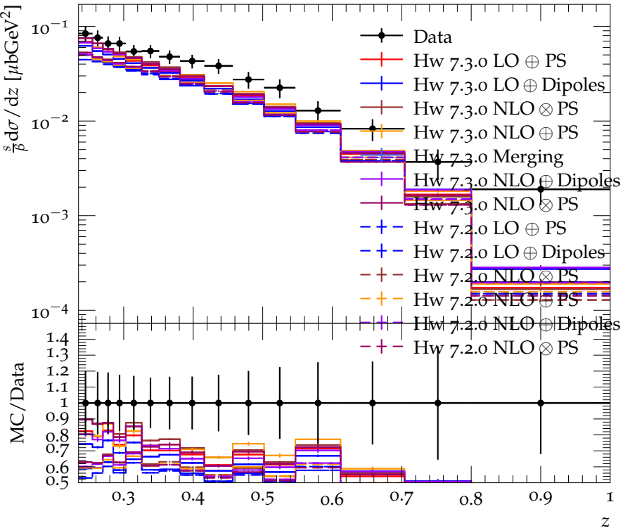
\phi spectrum in the continuum (10 GeV)
