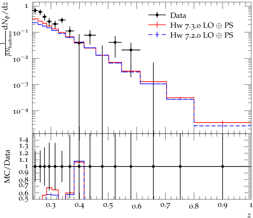
\phi spectrum in Y(2S) decays
