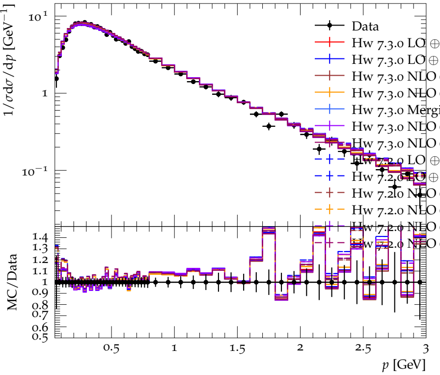
Spectrum of \pi^\pm in continuum (10 GeV)
