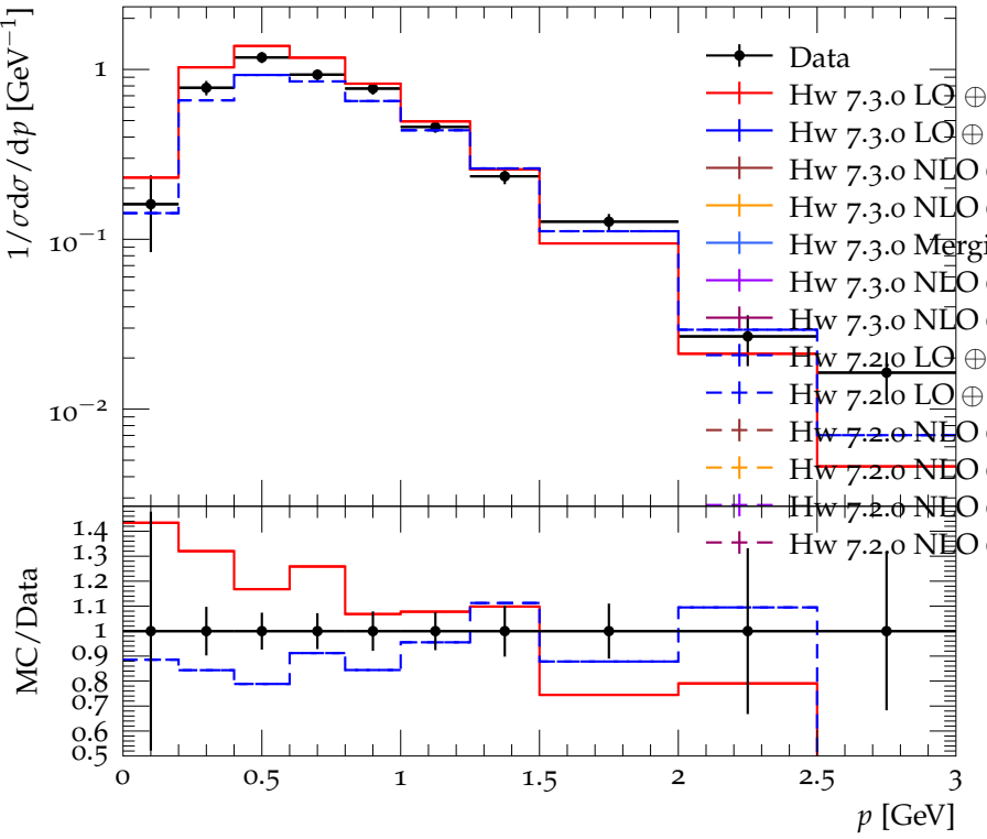
Spectrum of K_{S,L}^0 in Y(1S) decays
