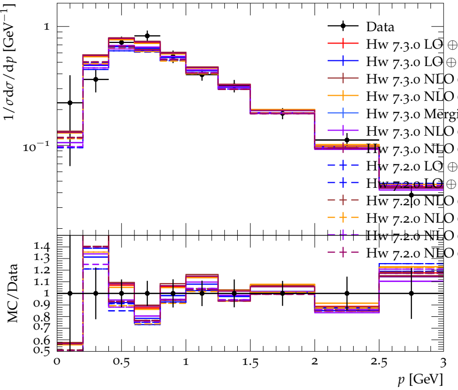
Spectrum of K_{S,L}^0 in continuum (10 GeV)
