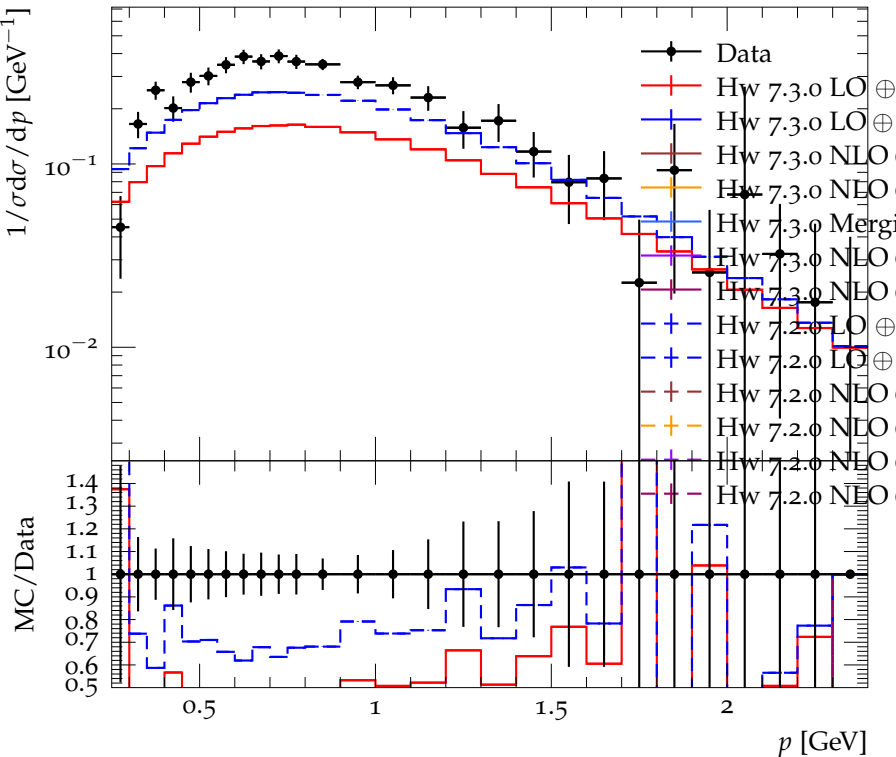
Spectrum of p, \bar{p} in Y(1S) decays
