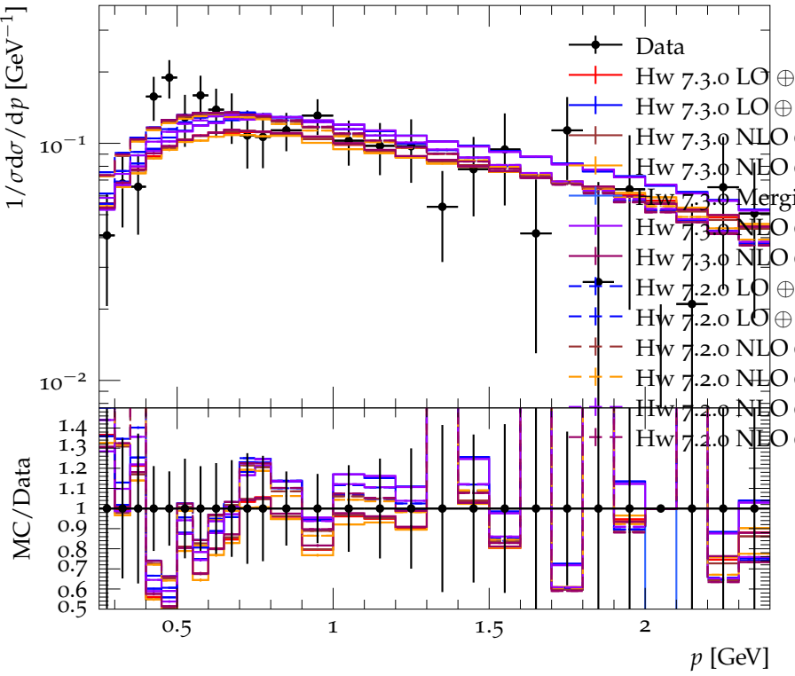
Spectrum of p, \bar{p} in continuum (10 GeV)
