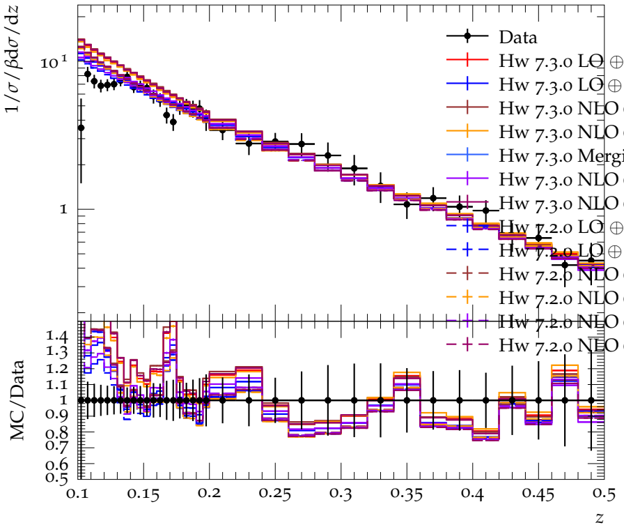
Spectrum of K^\pm in continuum (10 GeV)
