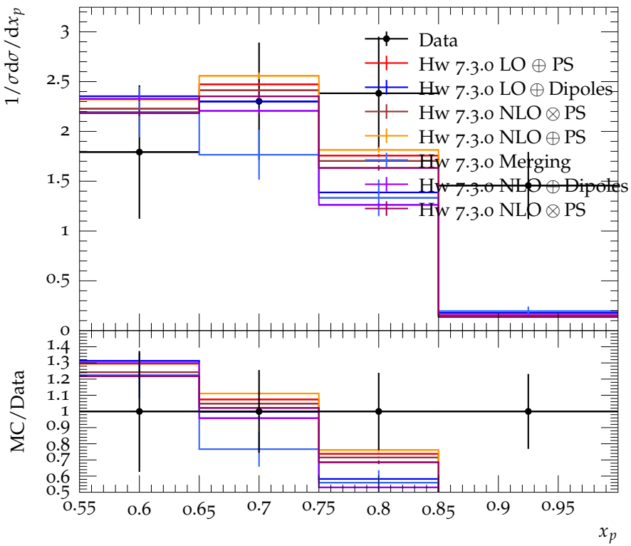
Scaled momentum spectrum for D_1(2420)^0
