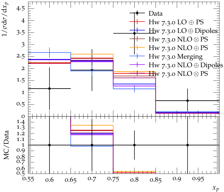
Scaled momentum spectrum for D_2^*(2460)^0
