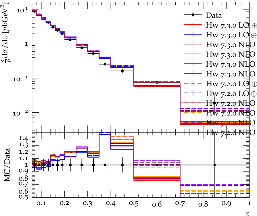
\pi^0 spectrum in the continuum (10 GeV)
