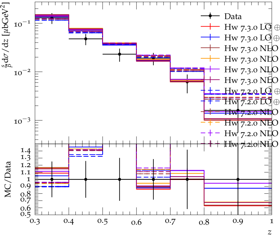
\eta spectrum in the continuum (10 GeV)
