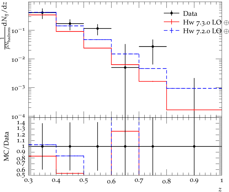
\eta spectrum in Y(2S) decays
