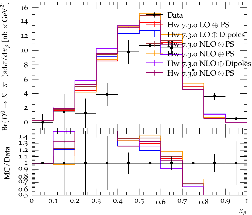
Scaled momentum spectrum for D^0, \bar{D}^0 production (continuum)
