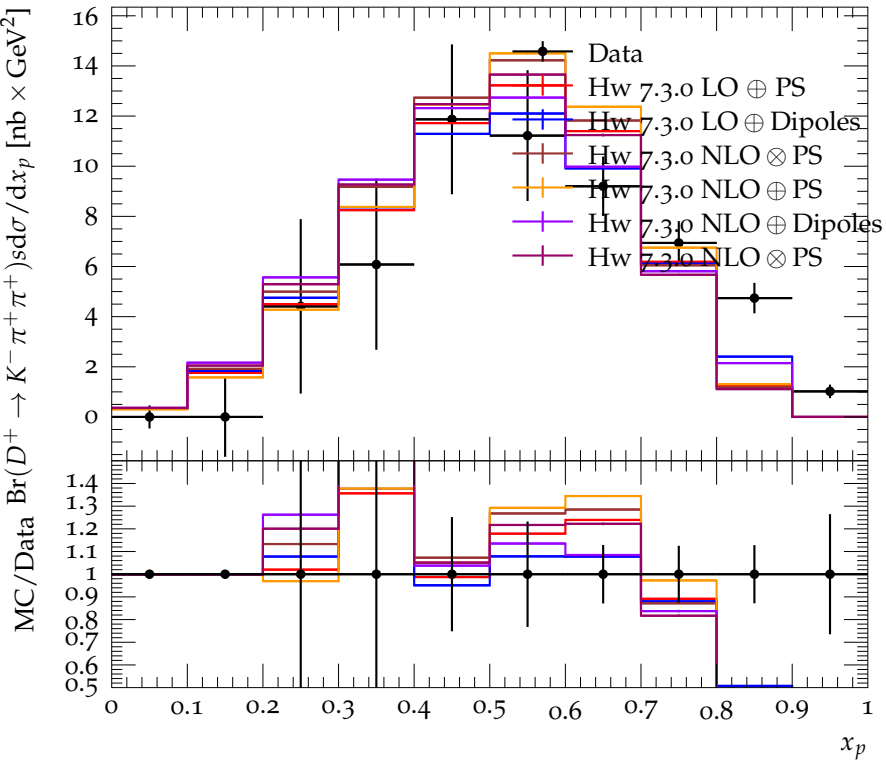
Scaled momentum spectrum for D^\pm production (continuum)
