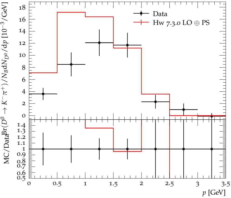
Momentum spectrum for D^0, \bar{D}^0 production (B decay)
