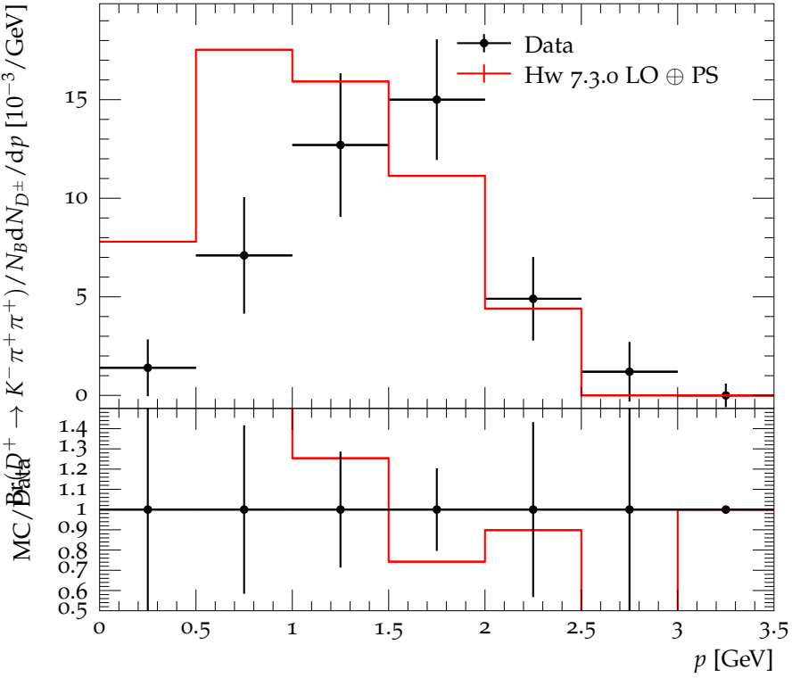
Momentum spectrum for D^\pm production (B decay)
