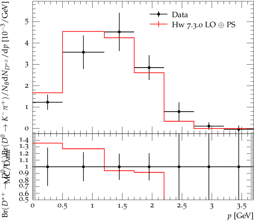
Momentum spectrum for D^{*\pm} production (B decay)
