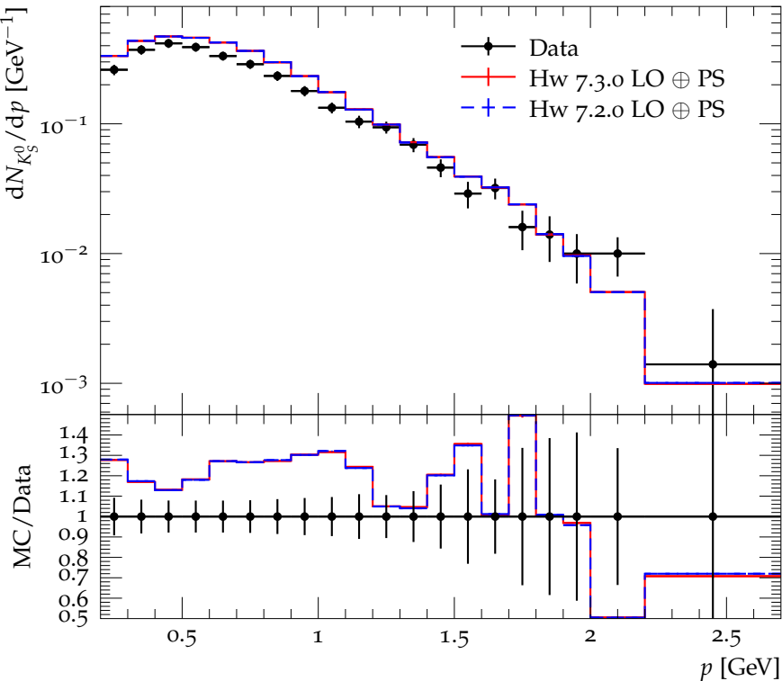
Number of K_S^0 per B decay as a function of momentum
