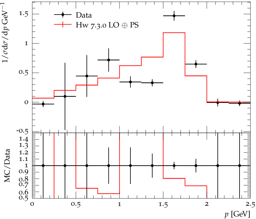
Momentum spectrum for D_s^{*+} at Y(4S)
